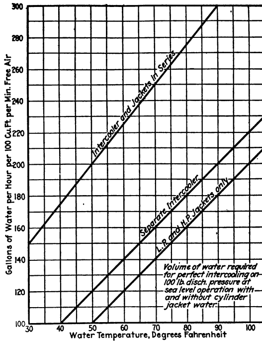
FIG. 62.—Water required for intercooling.
